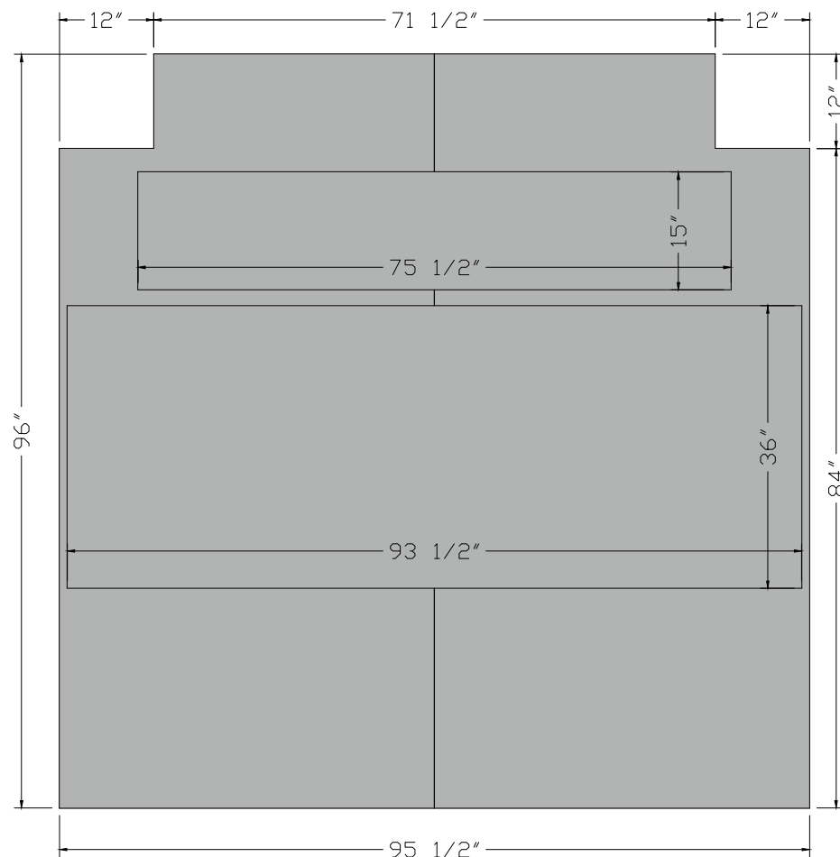
FACE VIEW
