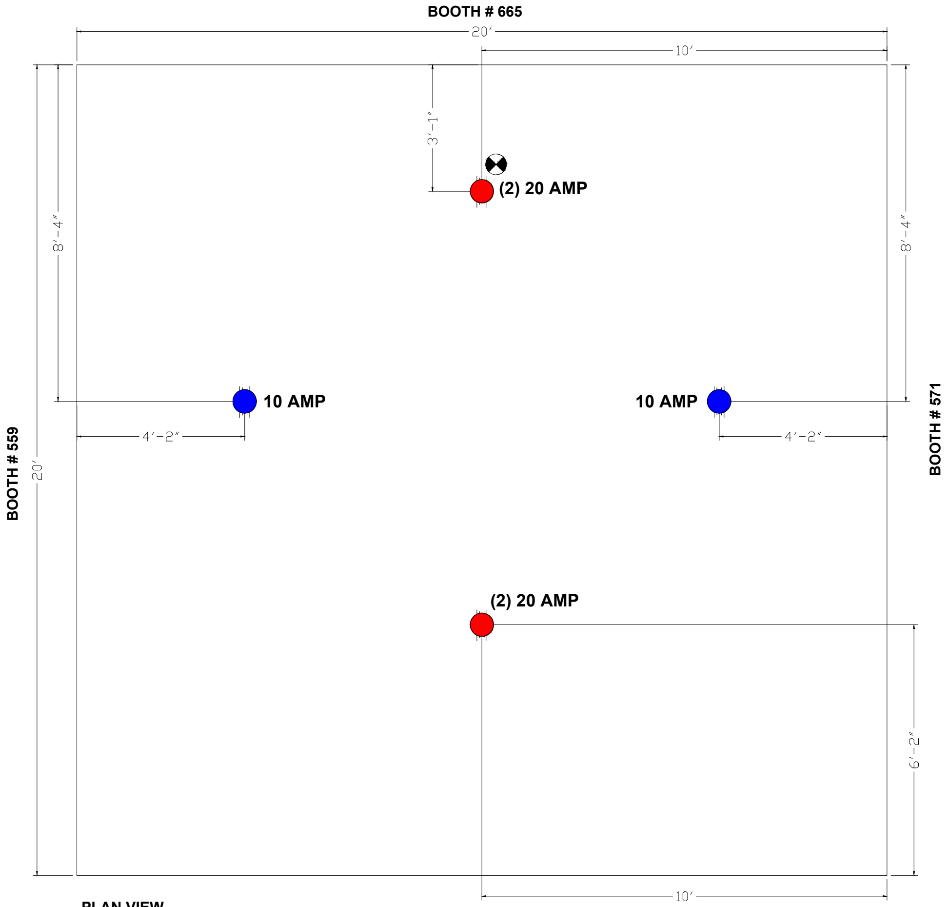
PLAN VIEW
