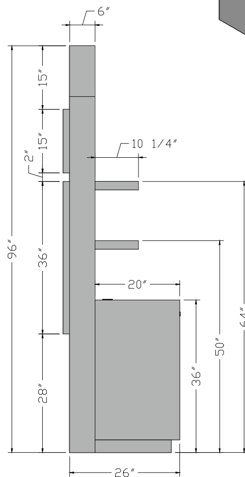
SIDE VIEW
