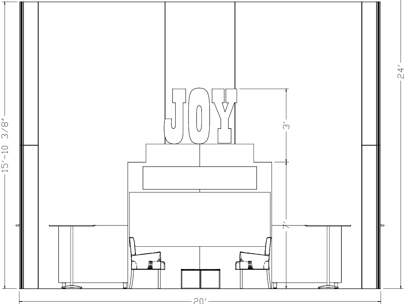
FACE VIEW
