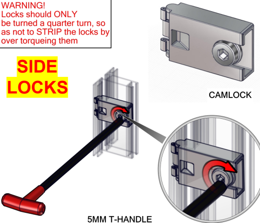
LOCK EXTRUSION BY USING 5MM HEX KEY
