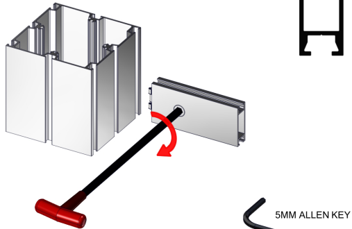
LOCK EXTRUSION BY USING 5MM ALLEN KEY
