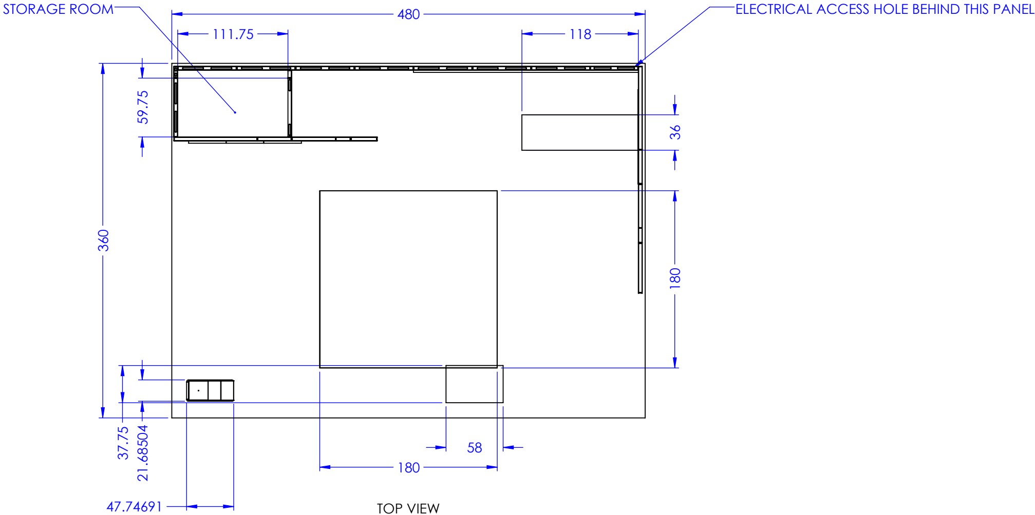
TOP VIEW
