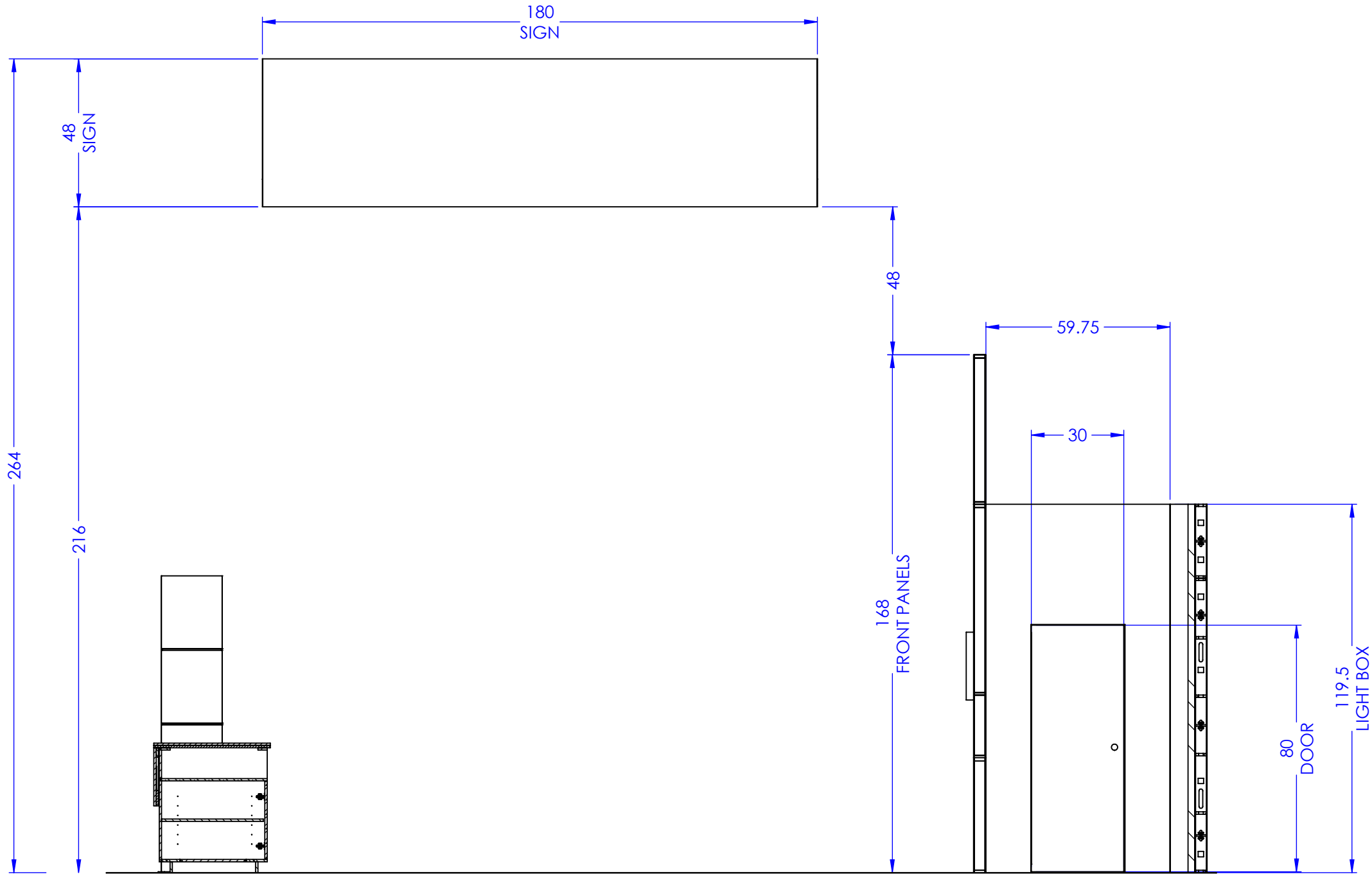
SECTION B-B
