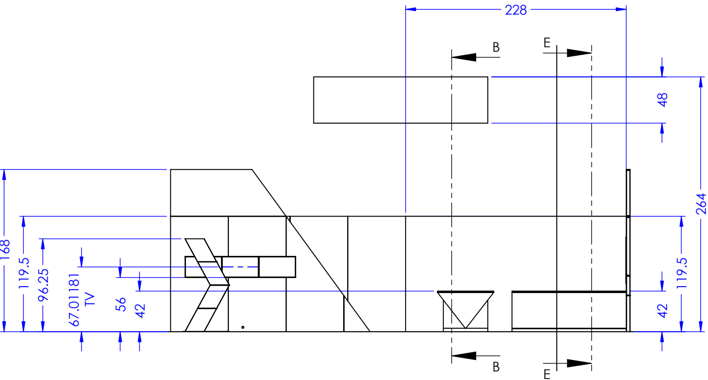
FRONT VIEW
