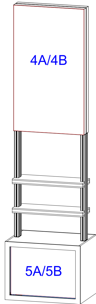
Kiosk - Qty. 3 Graphic Dims Scale 1:20 Add 1.5" Bleed to All Graphics
