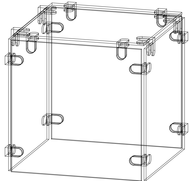
DETAIL VIEW OF GLASS CUBE
