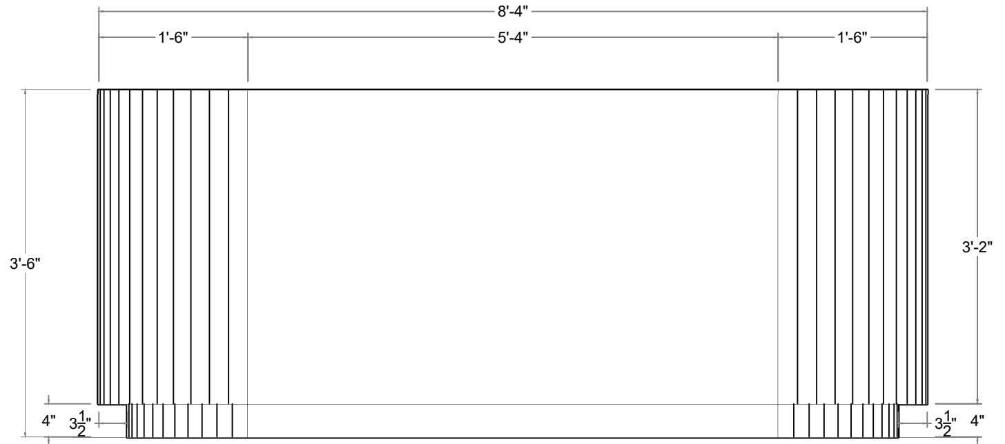
02 U SHAPED TABLE (FRONT VIEW) SCALE: 3/4" = 1'-0"
