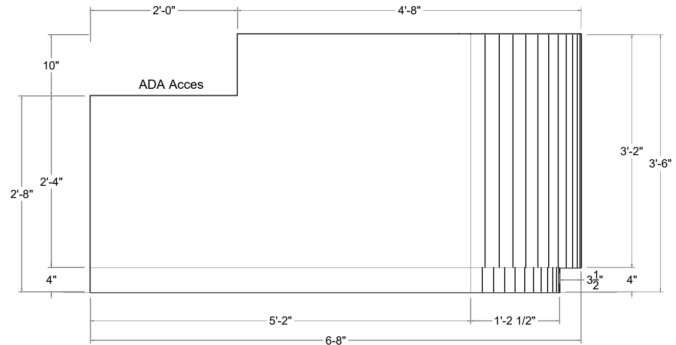
03 U SHAPED TABLE (SIDE VIEW) SCALE: 3/4" = 1'-0"
