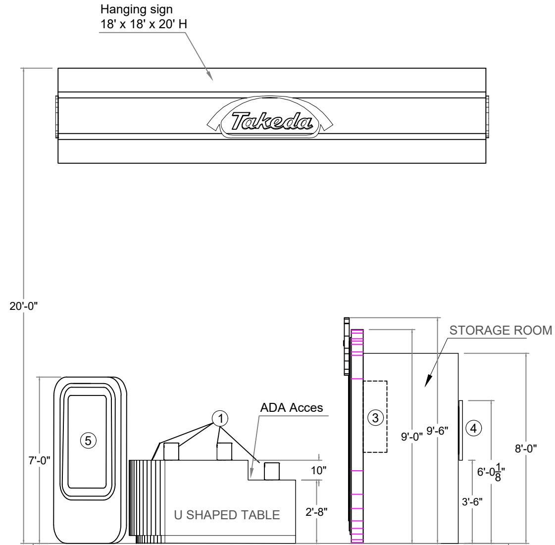
02 RIGHT SIDE VIEW SCALE: 1/4" = 1'-0"
