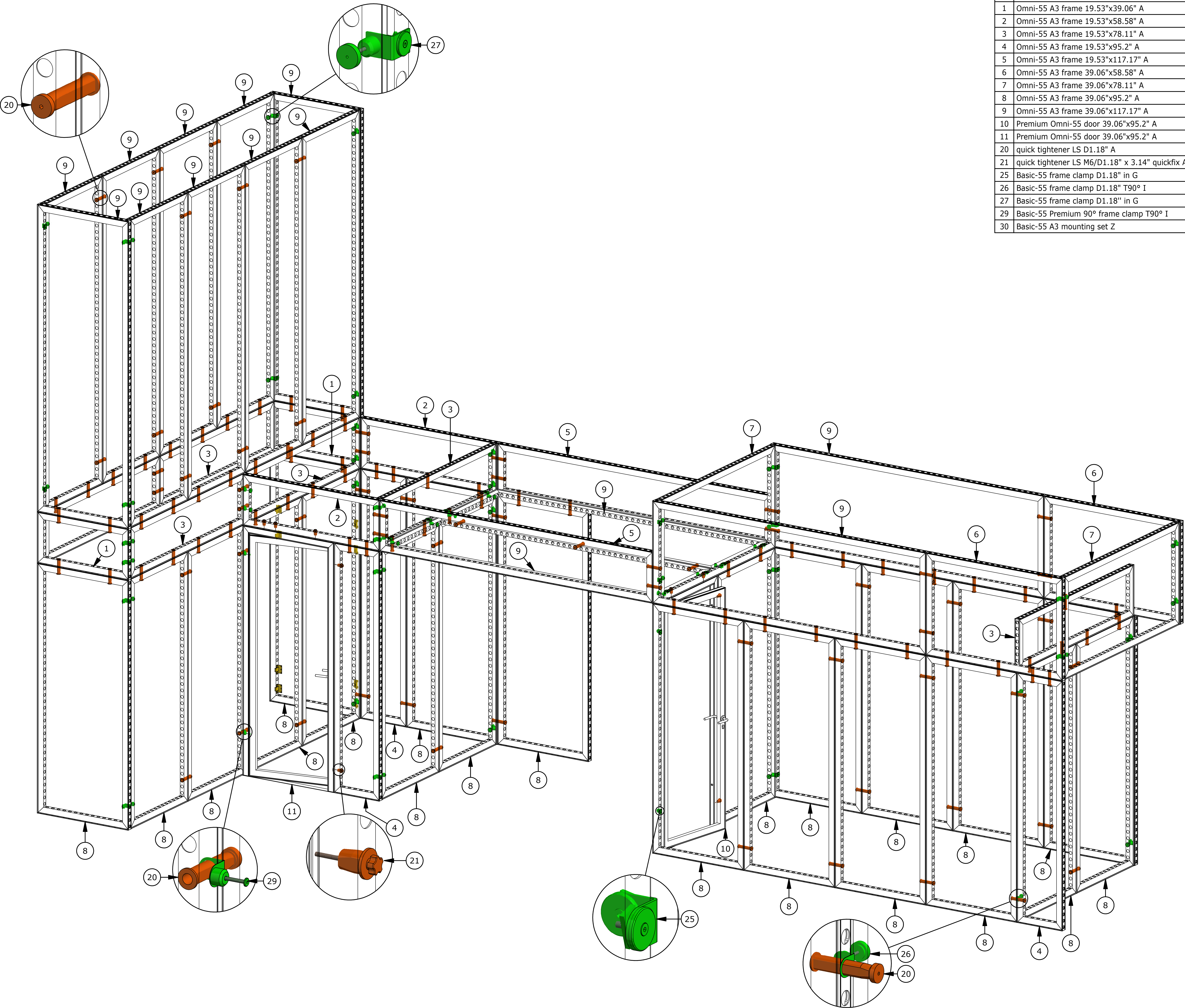
Main Structure
