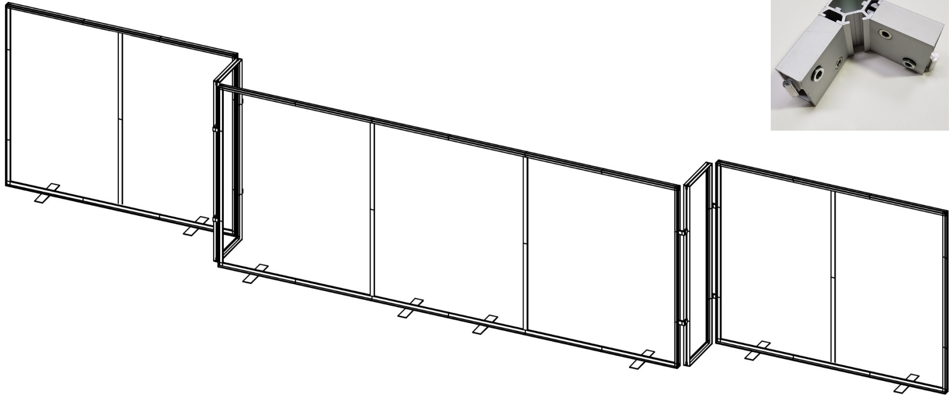
Corner Connector
